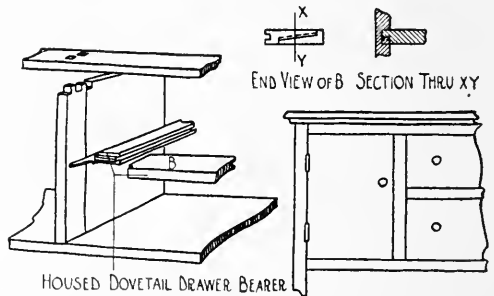
FIG. 428. DETAIL OF FRAMING DRAWER DIVISION.
